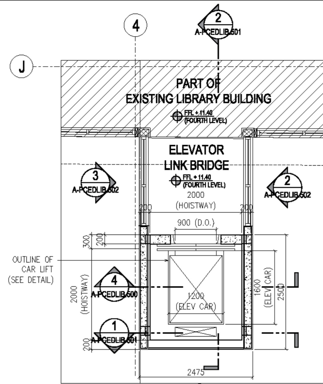
2 PCED LIBRARY BUILDING - ELEVATOR DETAIL SECOND - FOURTH FLOOR PLAN SCALE 1:50 20X30
