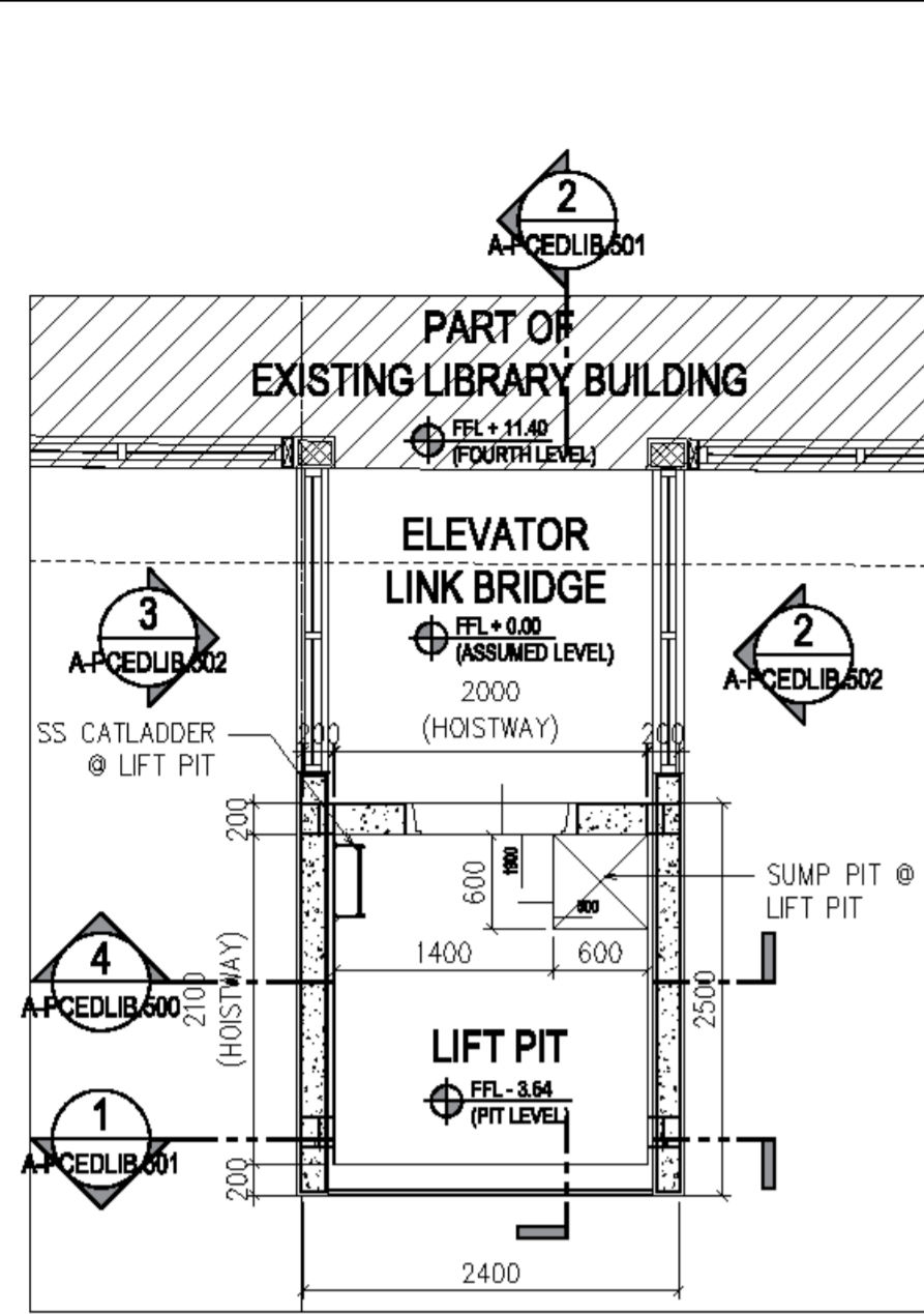
1 PCED LIBRARY BUILDING - ELEVATOR DETAIL GROUND FLOOR PLAN SCALE 1:50 20X30
