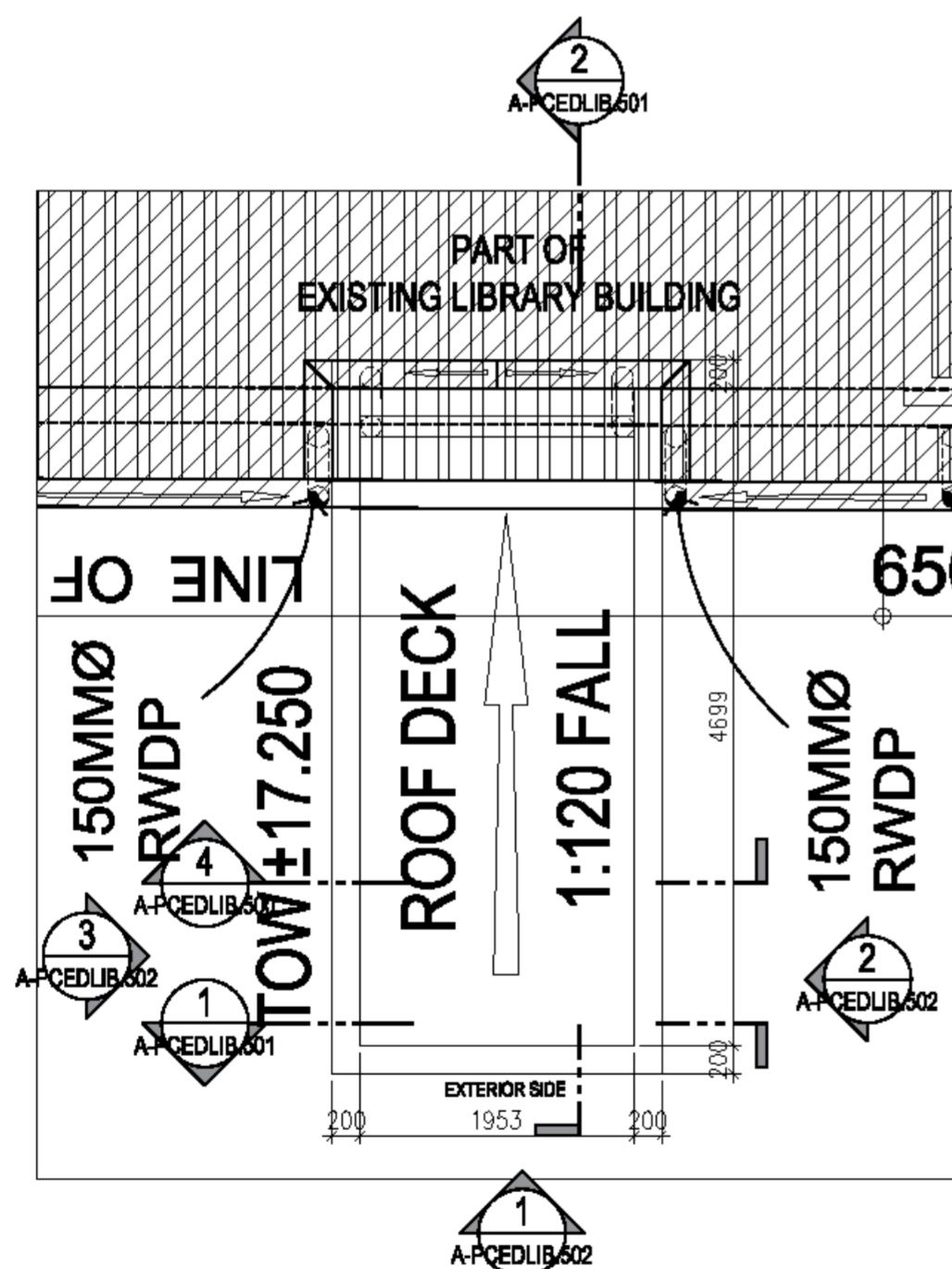
3 PCED LIBRARY BUILDING - ELEVATOR DETAIL ROOF PLAN SCALE 1:50 20X30
