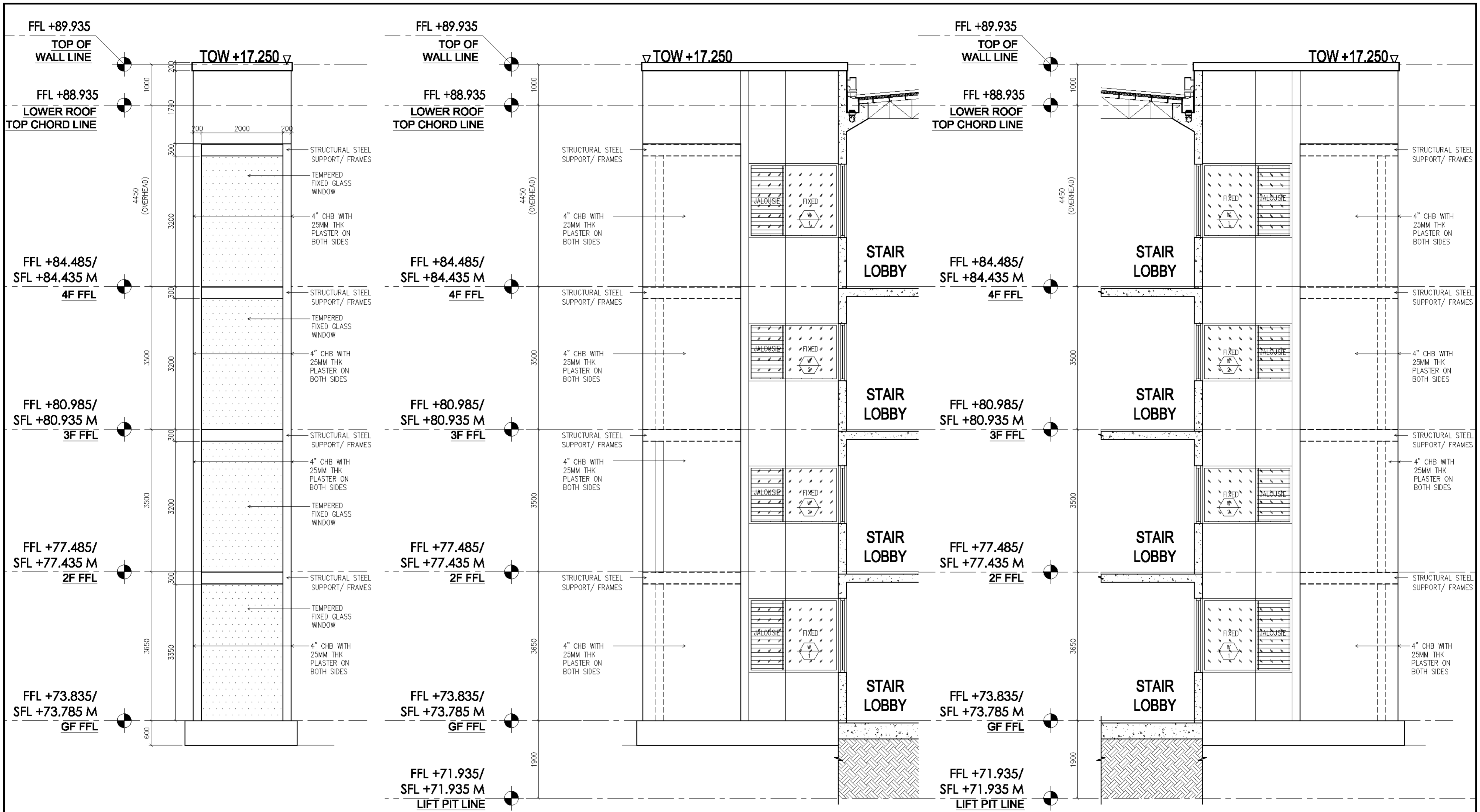
1 PCED LIBRARY BUILDING ELEVATOR FRONT ELEVATION SCALE 1:50 20X30
