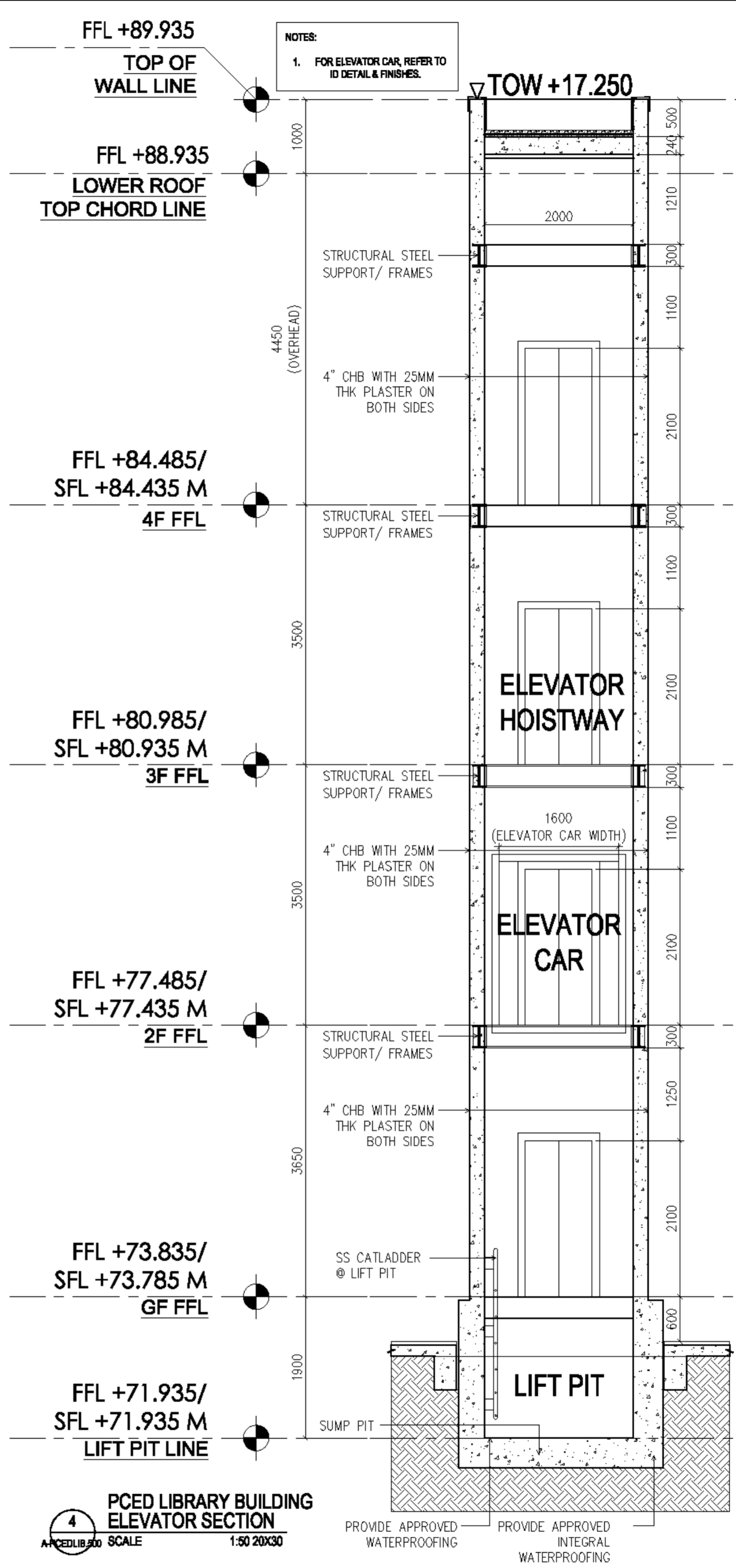
4 PCED LIBRARY BUILDING ELEVATOR SECTION SCALE 1:50 20X30
